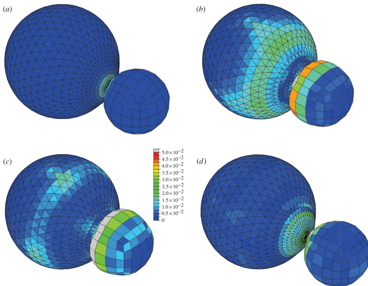
Figure 20. The pressure wave travelling through the eye in dynamic tonometry (units are N mm -2 ): (a) initial contact; (b) pressure wave; (c) dispersion of pressure wave; (d) pressure wave back at cornea following impact.
