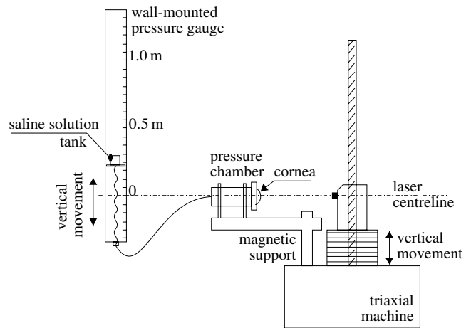
Figure 3. Trephinate inflation test rig.
